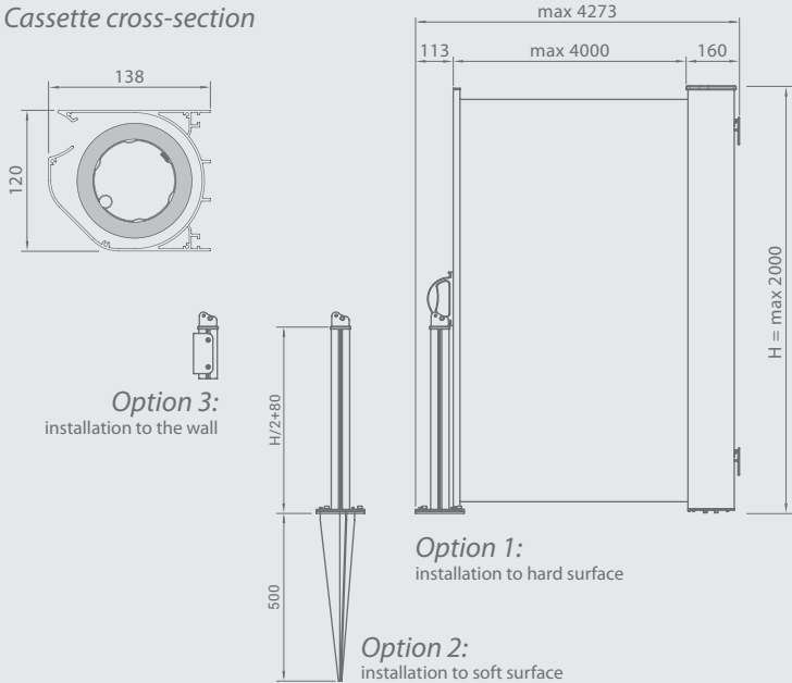
Cassette cross-section
